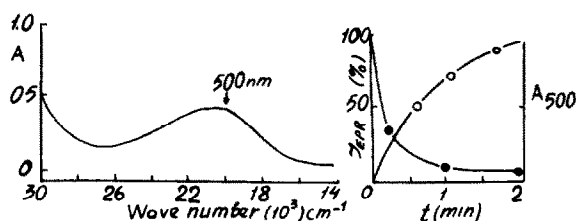
Fig.2. The optical spectrum of the product formed in the course of the reaction neurocuprein with adrenaline (left) and kinetic curves (right) for the drop of the EPR signal intensity (●) and the formation of the product (○)
