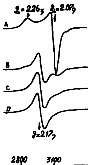
Fig.4 EPR spectra of neurocuprein after the addition of ferricyanide to the protein preliminarily reduced by adrenaline (A) and in the course of the titration of the reduced protein by adrenochrome. 0.5 (B), 1 (C) and 2 (D) equivalents of adrenochrome were added to the reduced protein.
